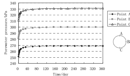
Fig. 7. Pore-water pressure around the lining (with permeable advance face and impermeable lining. T = 0 refer to the end of the tunnel excavation).
