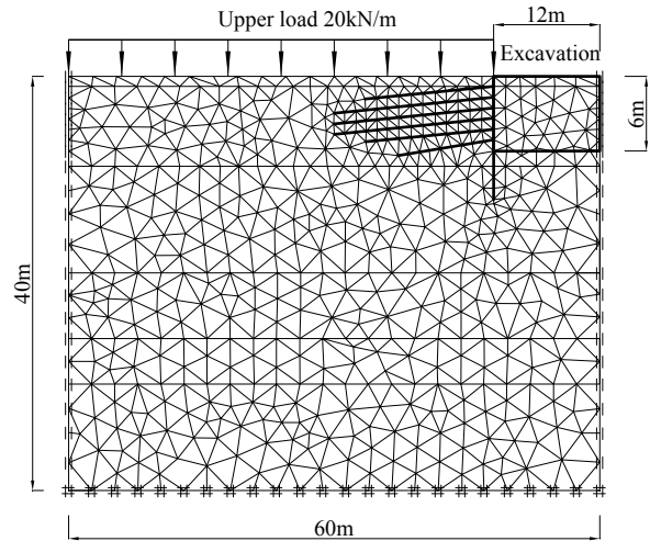
Fig. 4 The finite element model
