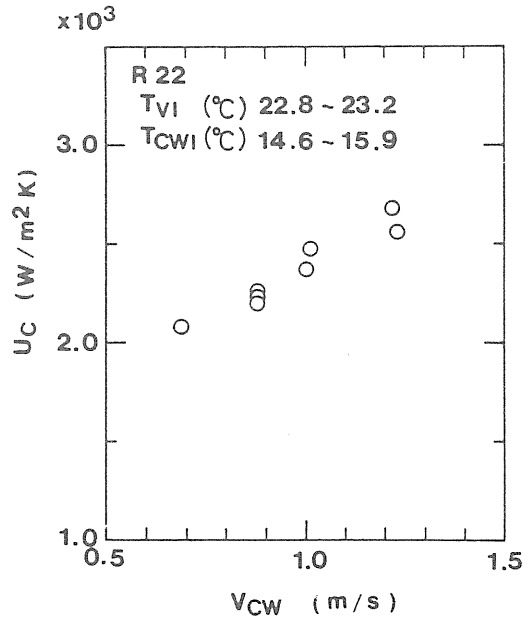
Fig. 6 Overall heat transfer coefficient U_c for condenser versus velocity of the cold water V_{cw}
