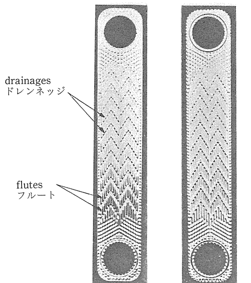
(a) Working fluid side (b) Water side
