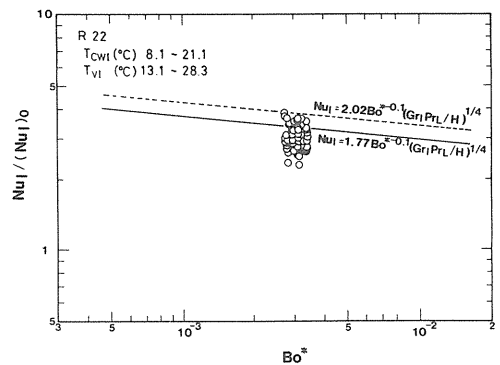
Fig. 9 Nu_i / \{(Nu_i)_0\} \sim Bo^*
