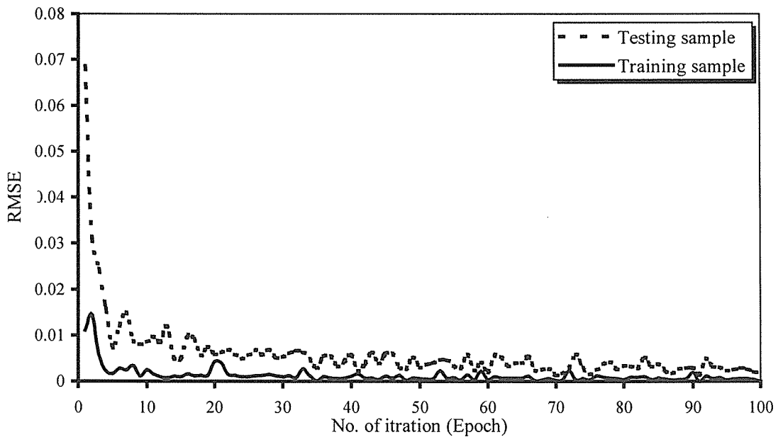
Fig. 3 Root mean square error (RMSE) in back propagation learning
